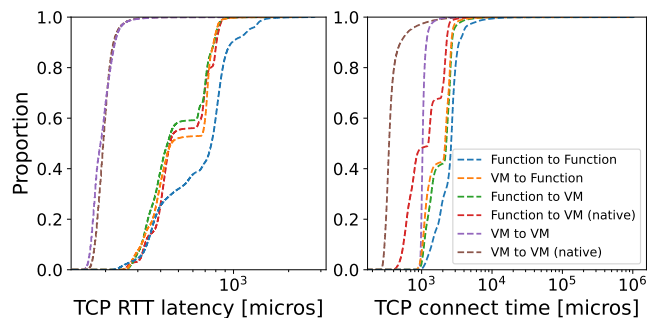
Figure 8. Empirical CDF of RTT latencies (left) and TTFB TCP connection establishment times (right) between different types of connecting and accepting hosts running Boxer or without (native).
